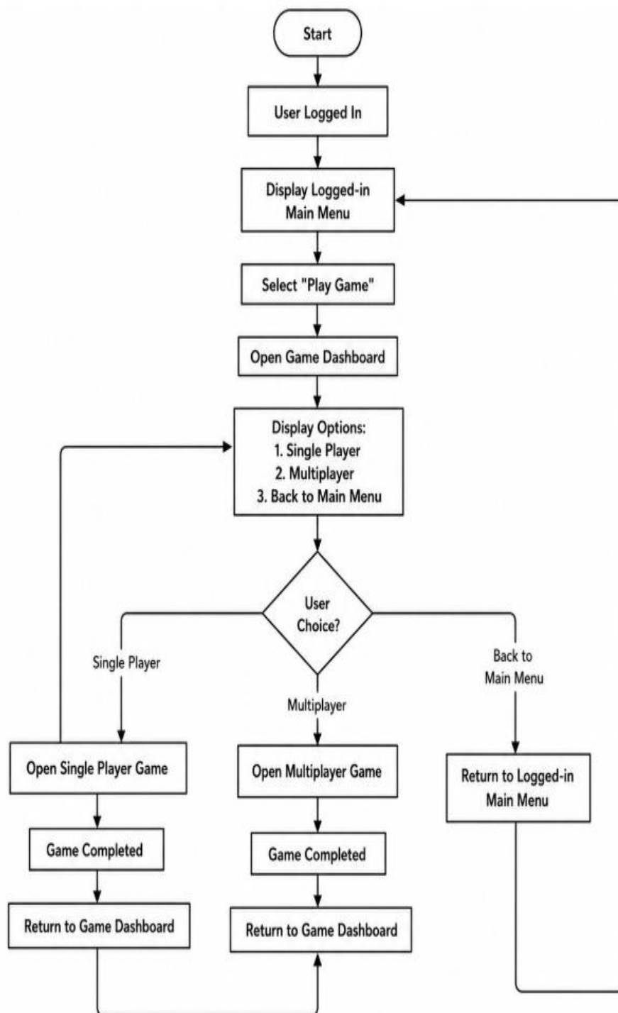
Figure 6.4 : Flowchart for Dashboard
